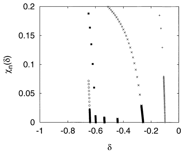
Figure 13. The same as figure 12 but for the second moment of the kink density. It is also apparent here that the value of \delta_c(h) , being equal to 0.70(1) for h = 0.1 according to simulations, is fairly well approximated by the GMF results for N = 5, 6 .
