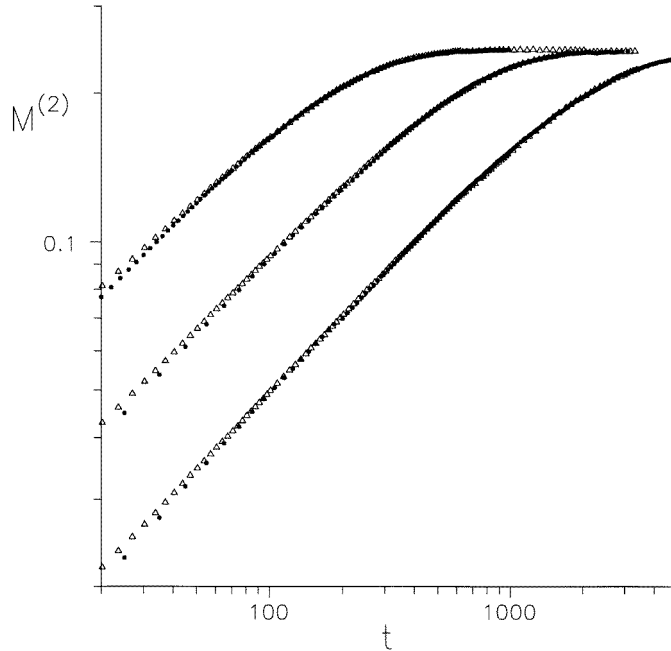
Figure 8. M^{(2)}(t, L) with APBC. Rescaling with b = 2 , \beta = 0 and Z = 1.75 has resulted in data points marked by \Delta . Collapsing of curves is shown, from top to bottom, for L = 32 ( \Delta ), 64 ( \bullet ); 64 ( \Delta ), 128 ( \bullet ); 128 ( \Delta ), 256 ( \bullet ). Number of samples in averaging: 10^5 – 3 \times 10^5 .
