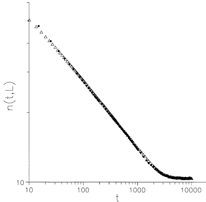
Figure 7. Collapsing of curves for n(t, L) according to equation (16). \triangle : L = 100 , rescaled; \bullet : L = 200 . Number of samples in the averaging: 10^5 . Boundary condition: antiperiodic; scale: double-logarithmic.
