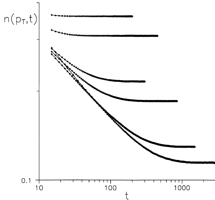
Figure 3. The kink-density as a function of temperature and time n(p_T, t) . The curves are for p_T = 10^{-1}, 5.0 \times 10^{-2}, 10^{-2}, 5.0 \times 10^{-3}, 10^{-3}, 5.0 \times 10^{-4} from top to bottom. L = 2000 and the number of samples in averaging is typically 2 \times 10^4 .
