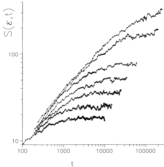
Figure 2. The structure factor S(\epsilon, t) in the active phase in the vicinity of the PC transition point for the following values of \epsilon : 0.13, 0.11, 0.09, 0.075, 0.06, 0.04, 0.03 (from bottom to top). L was varied between 2000 and 8000 to avoid finite-size effects before saturation sets in. The number of independent states in averaging is typically 1000.
